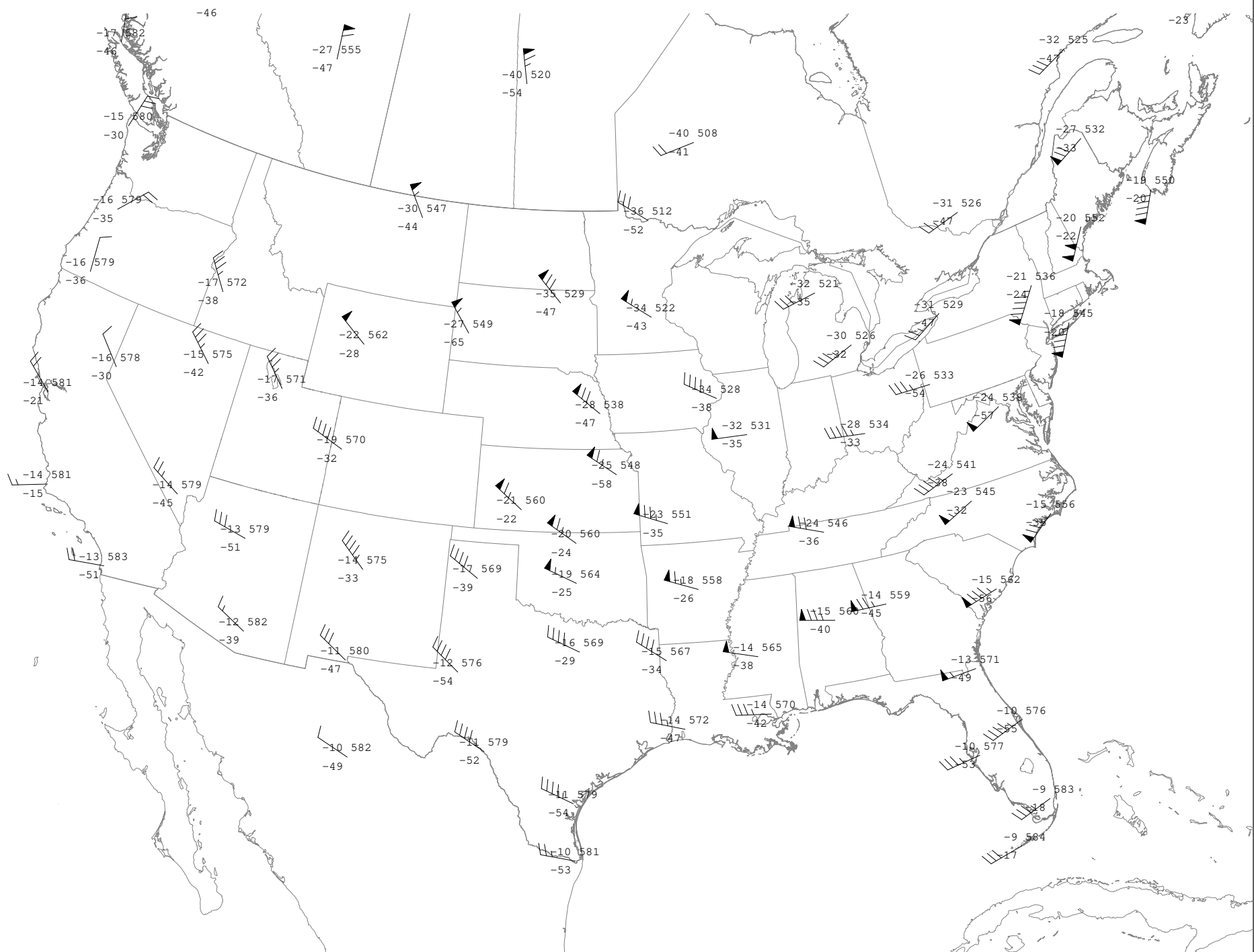
500 mb Observations Valid 260119/0000 UTC College of DuPage NEXLAB
