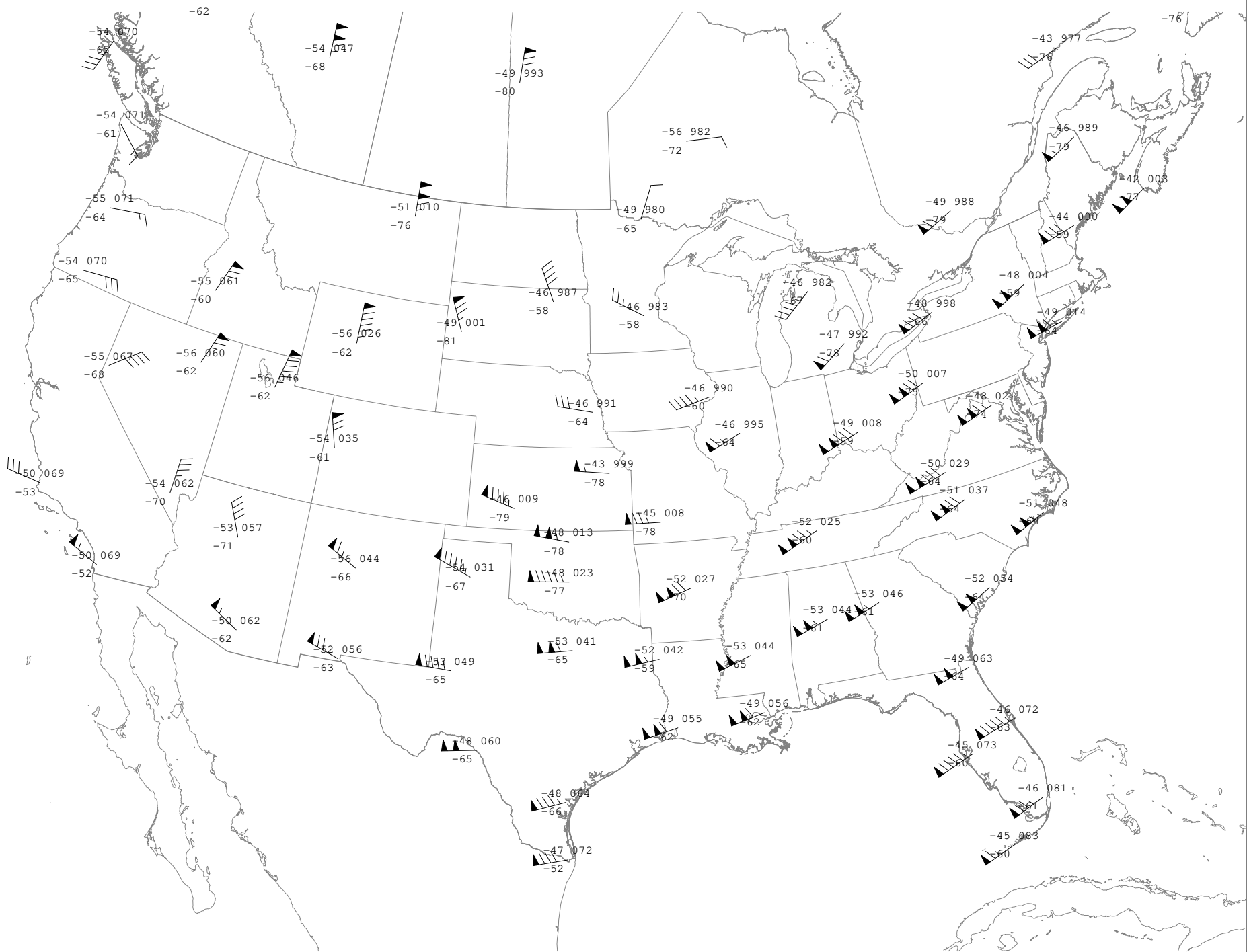
250 mb Observations Valid 260117/0000 UTC College of DuPage NEXLAB
