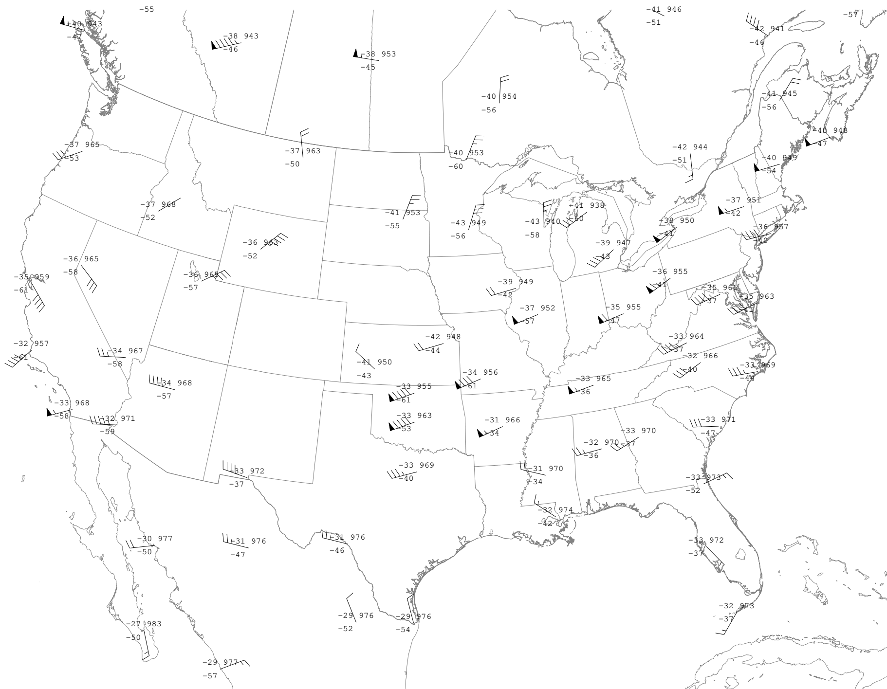
300 mb Observations Valid 250924/1200 UTC College of DuPage NEXLAB
