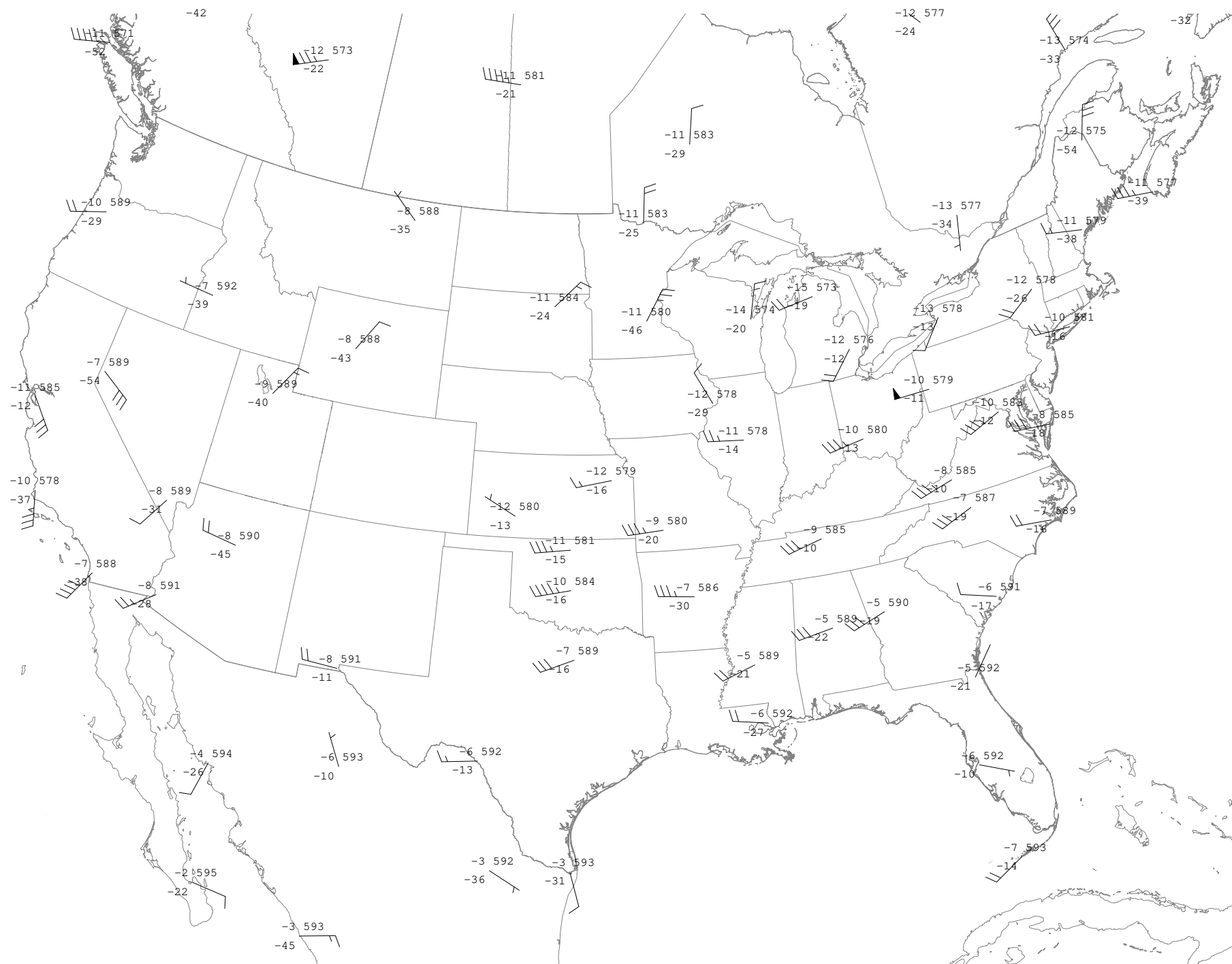
500 mb Observations Valid 250924/1200 UTC College of DuPage NEXLAB
