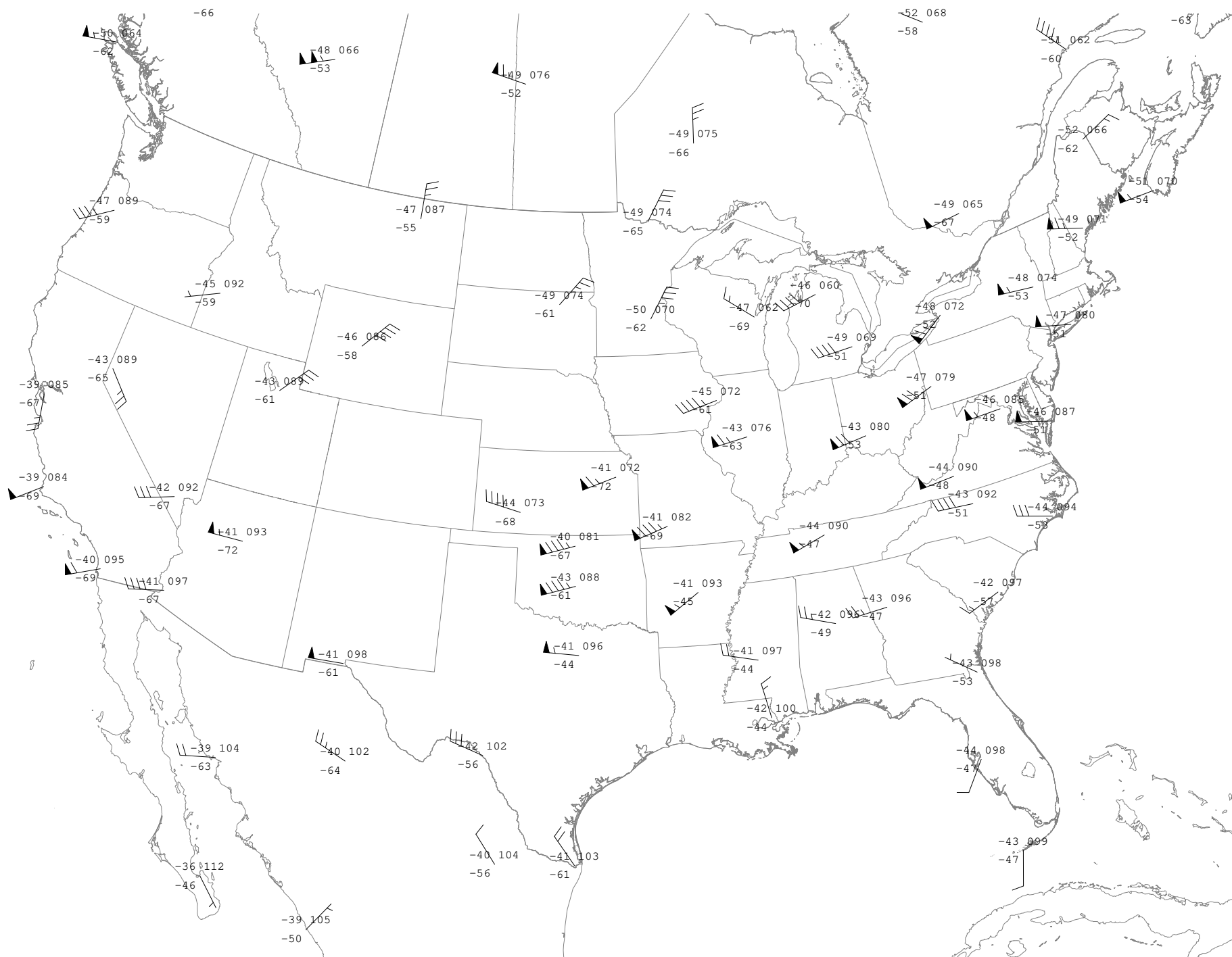
250 mb Observations Valid 250924/1200 UTC College of DuPage NEXLAB
