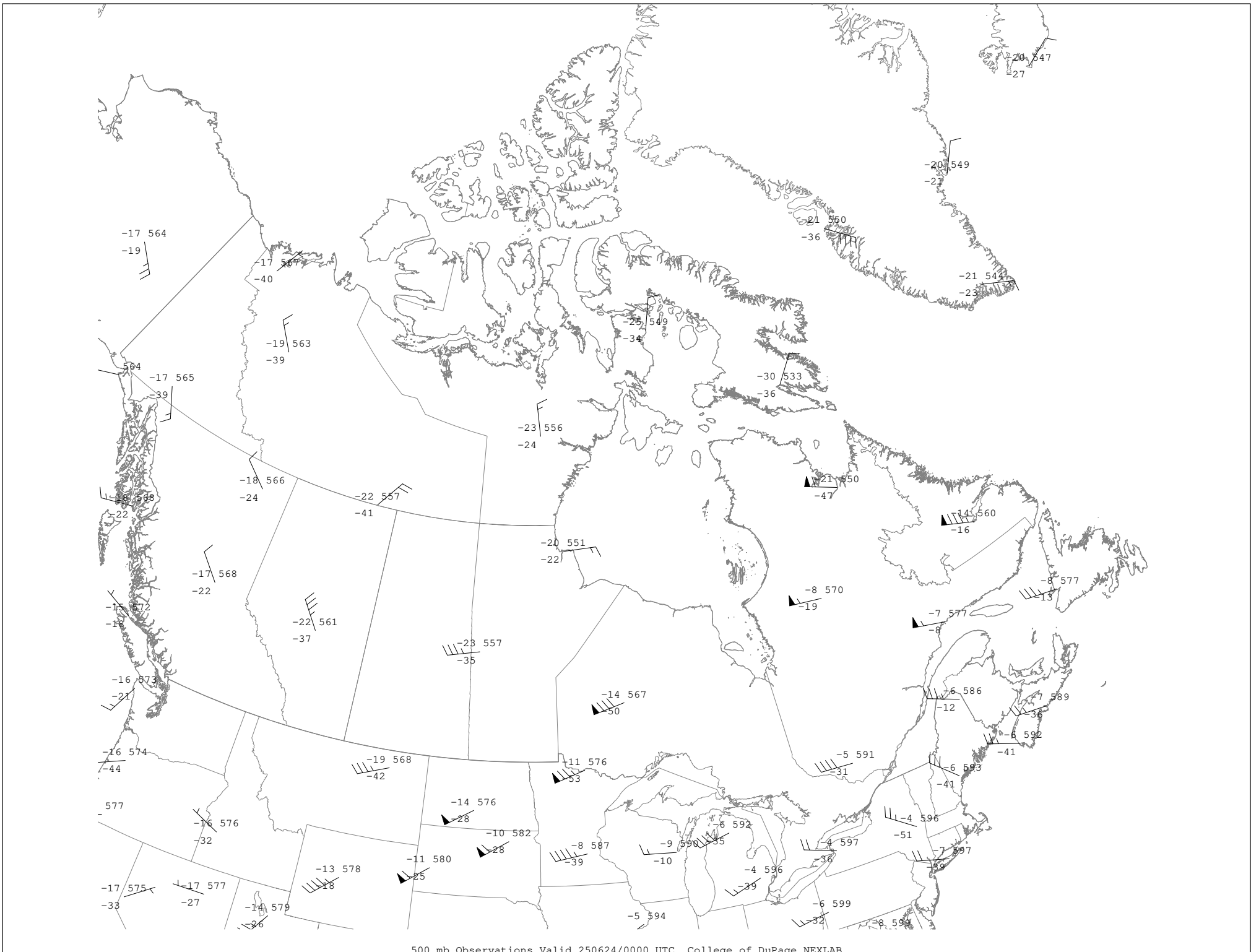
500 mb Observations Valid 250624/0000 UTC College of DuPage NEXLAB
