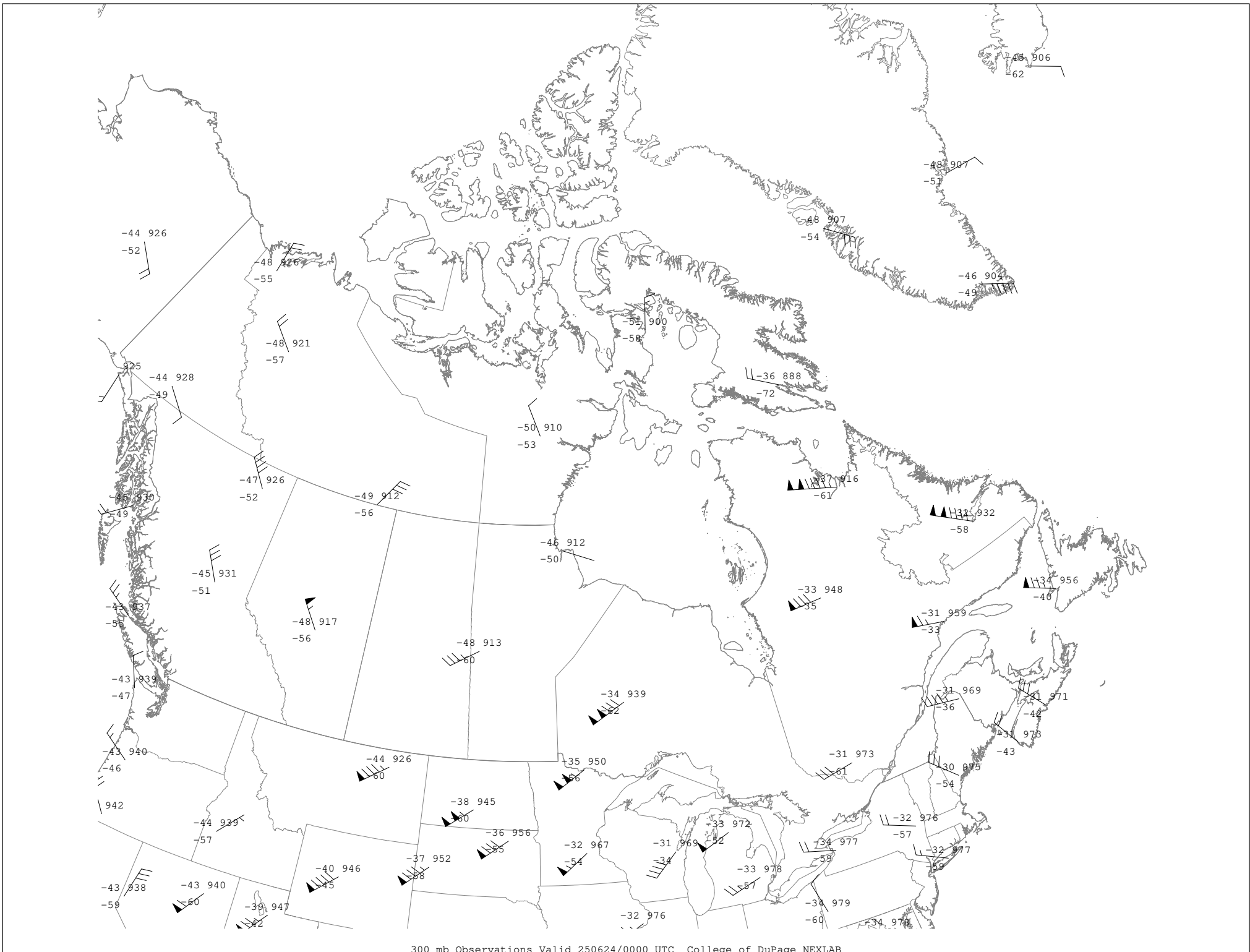
300 mb Observations Valid 250624/0000 UTC College of DuPage NEXLAB
