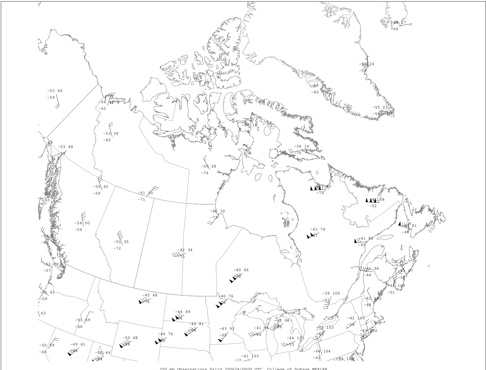
250 mb Observations Valid 250624/0000 UTC College of DuPage NEXLAB
