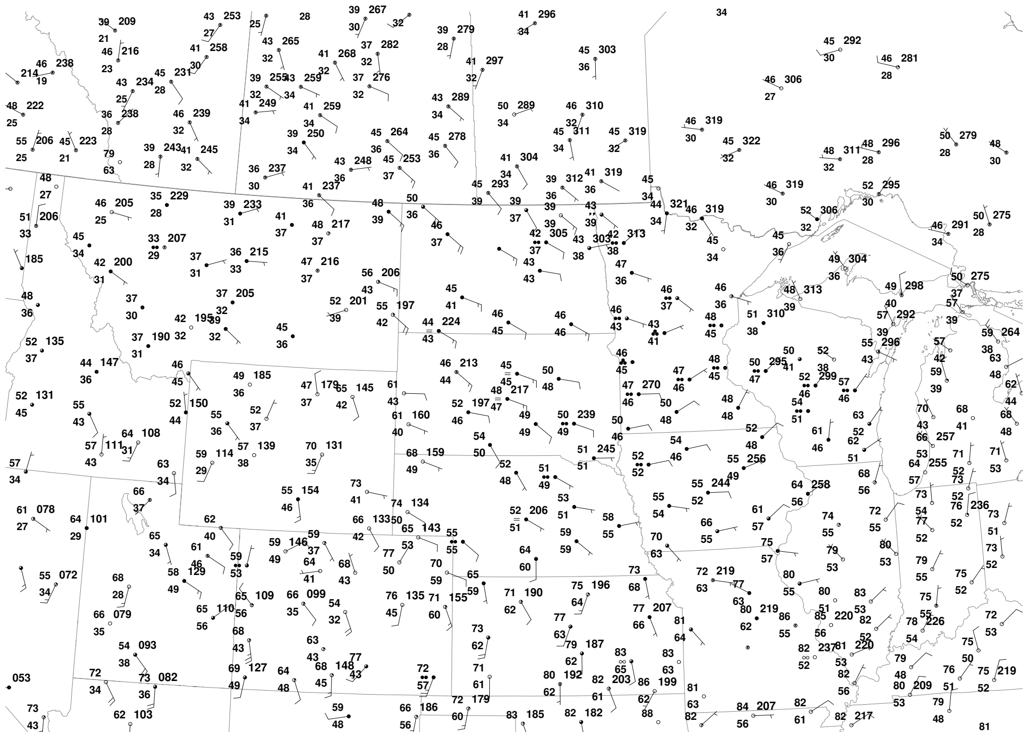
251014/2100 COD NEXLAB SURFACE PLOT
