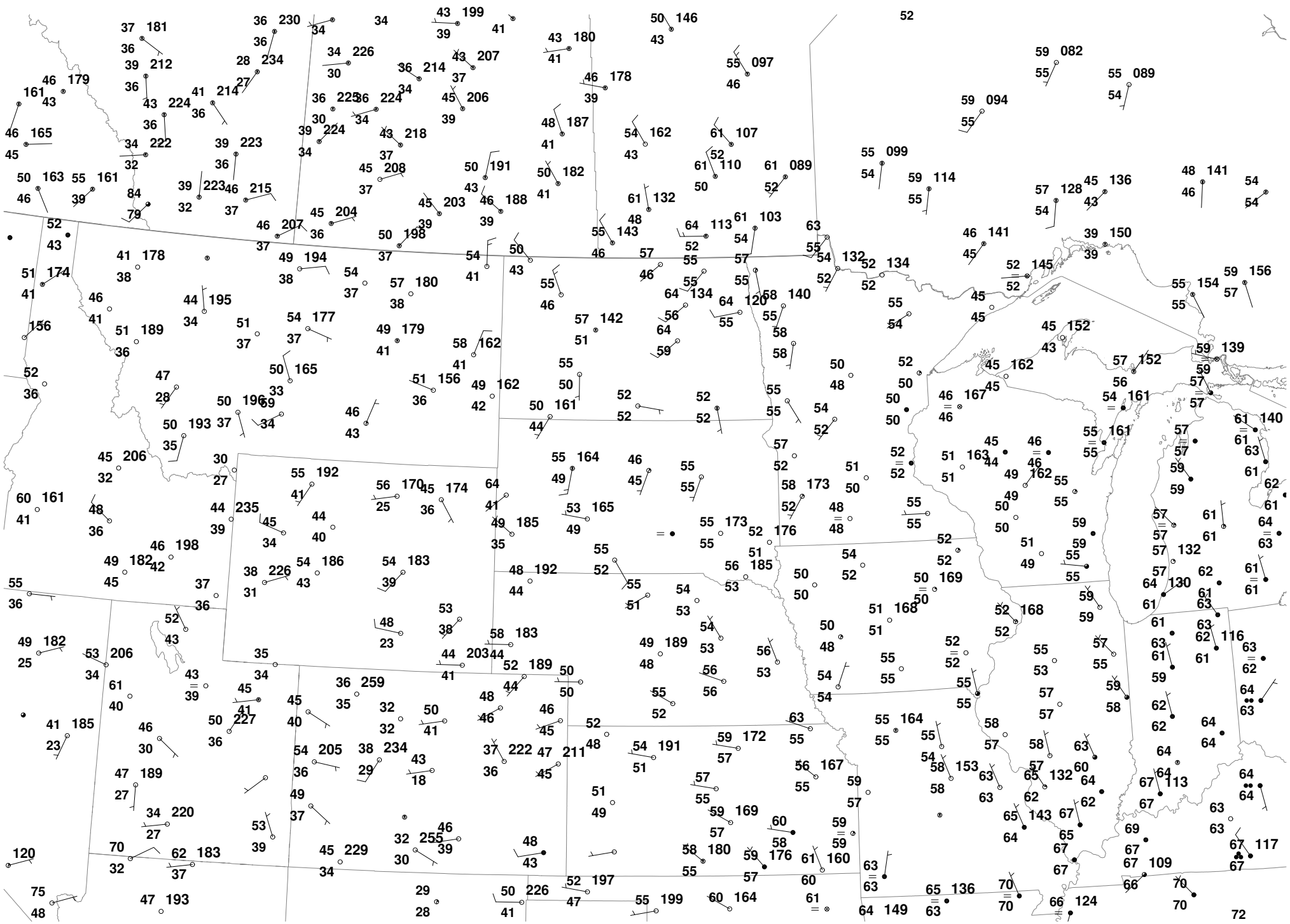
250925/0900 COD NEXLAB SURFACE PLOT
