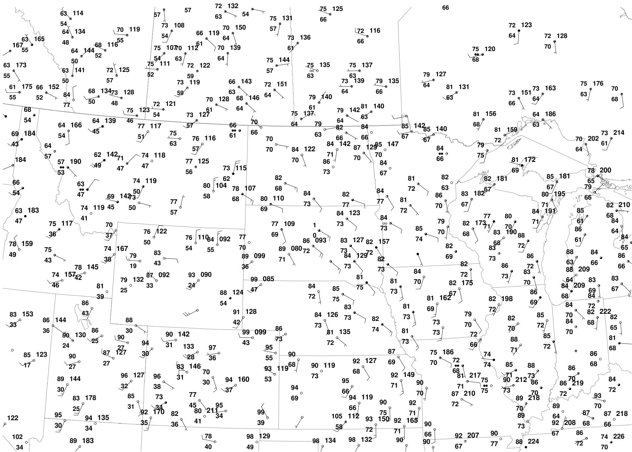
250807/1800 COD NEXLAB SURFACE PLOT
