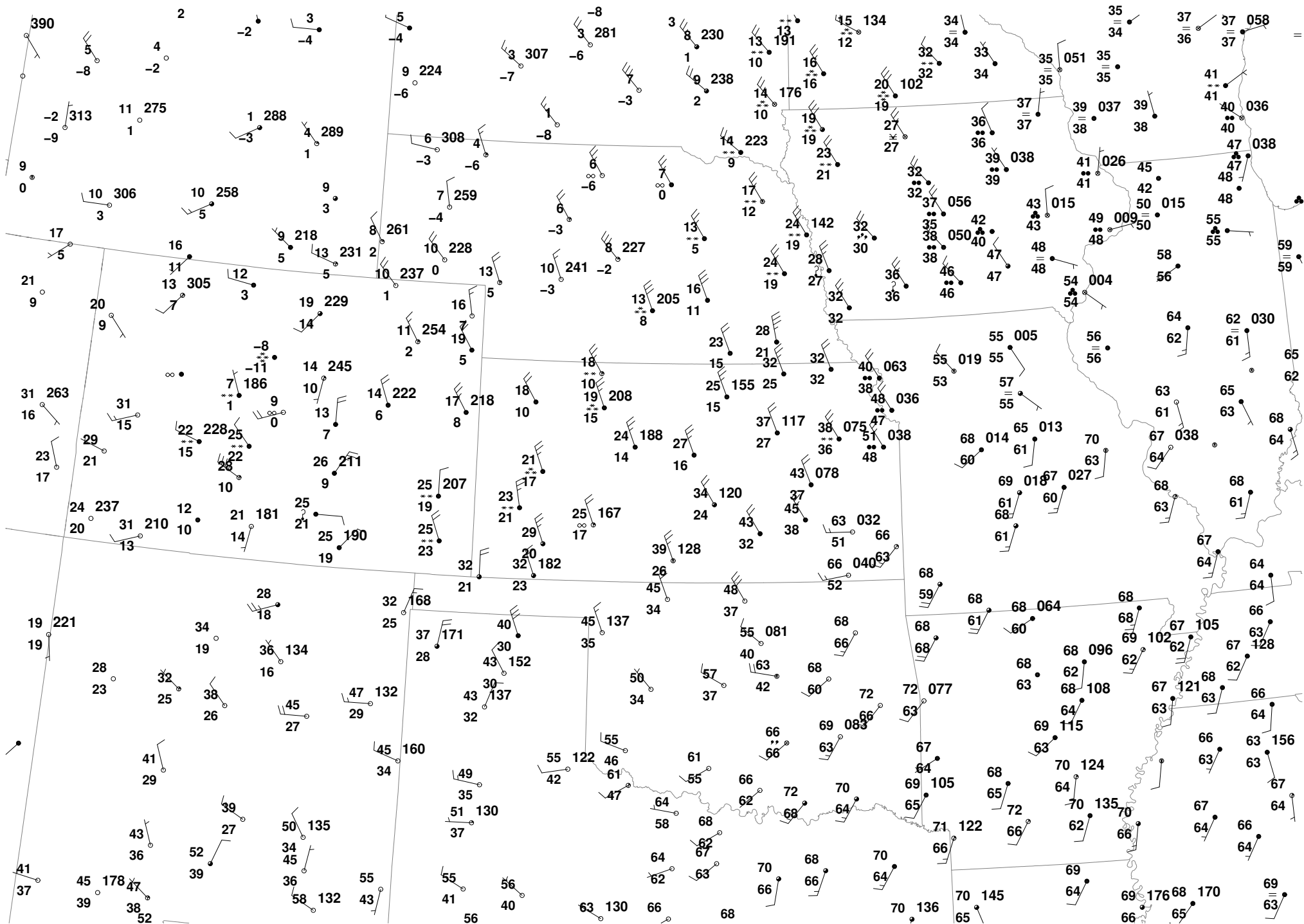
251228/1500 COD NEXLAB SURFACE PLOT
