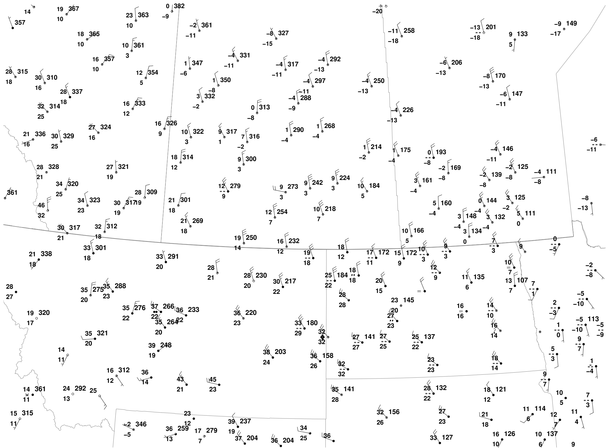
260118/1300 COD NEXLAB SURFACE PLOT
