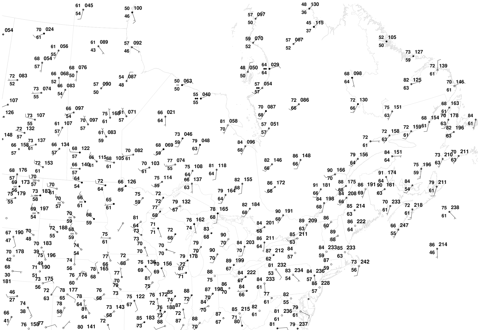
250810/1700 COD NEXLAB SURFACE PLOT
