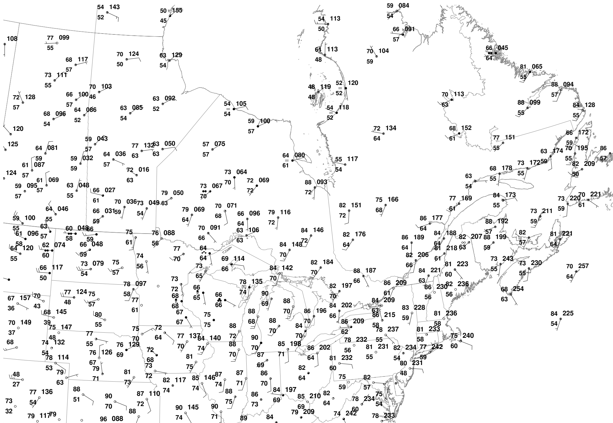
250809/1700 COD NEXLAB SURFACE PLOT
