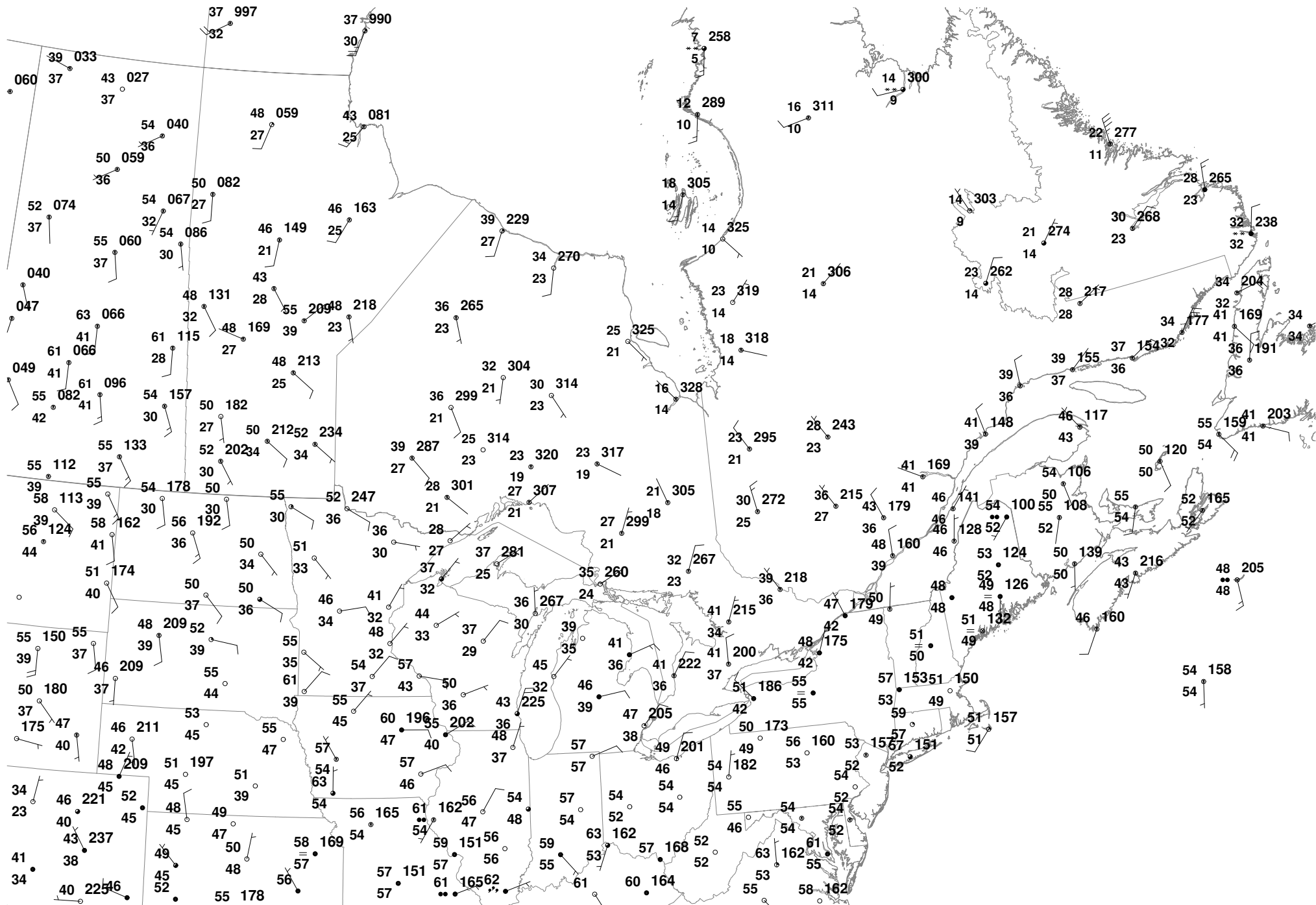
250508/0600 COD NEXLAB SURFACE PLOT
