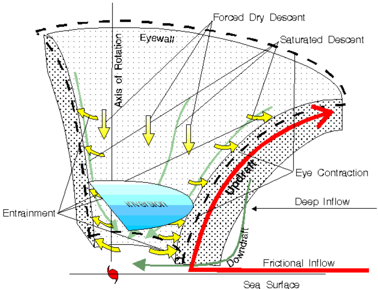
Schematic illustration of the secondary flow around the eye of a hurricane. The frictional updraft feeds the buoyancy-driven primary updraft and outflow in the eyewall cloud. Saturated convective downdrafts in the eyewall and the evaporatively driven descent along the inner edge of the eyewall feed moist air into the volume below the inversion surface. Dynamically driven descent of dry air inside the eye warms the air column adiabatically. The descent is forced as entrainment into the eyewall draws mass from the bottom of the eye into the eyewall. Balance between moist-air production and loss by entrainment determines the rate of rise or fall of the inversion. (From Atlantic Oceanographic and Meteorological Laboratory (AOML) web site, http://www.aoml.noaa.gov/ )
